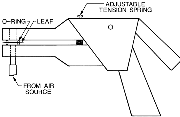
FIG. 22.8 A mass flow porometer. The basic structural material consists of plexiglass cemented together. The critical aspect in construction is alignment of the cup (cut from the two O-rings, both horizontally and vertically). Alignment of the two arms of the cup (cut from 1.3-cm-thick plexiglass sheets) is ensured by fixing, with a close-fitting metal pin, the upper arm snugly between the two large parallel trapezoidal plates glued to the lower arm. One O-ring is glued to an arm first. The other arm is then sanded to ensure good horizontal alignment of the O-rings. Vertical alignment is effected when the second O-ring is glued onto the arm. (From Hsiao, T.C., and Fischer, R.A., Mass flow porometers. In Measurement of Stomatal Aperture and Diffusive Resistance (Kanemasu, E.T., Ed.) ©1975 Bulletin 809, College of Agriculture Research Center, Washington State University: Pullman, Washington. Reprinted by permission of the Director of the Washington State University Agricultural Research Center, Pullman, Washington.)
