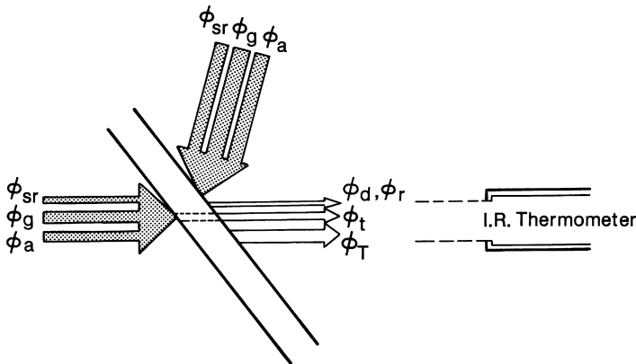
FIG. 24.2 Scheme of fluxes of energy on a surface like a leaf. \phi_r : energy emitted by the surface; \phi_g : part of global radiation received by the surface; \phi_a : part of long-wave radiation emitted by sky and received by the surface; \phi_{sr} : radiation from the surroundings received by the surface; \phi_r : reflected part of all these radiations; \phi_d : diffused part of all these radiations; \phi_t : transmitted part. (From Perrier, A., Leaf temperature measurement. In Plant Photosynthetic Production. Manual of Methods , p. 632-671, ©1971, Z. Šesták, J. Čatský, and P.G. Jarvis, Eds. Fig. 17.7c, p. 656. Dr W. Junk N.V.: The Hague, The Netherlands. With kind permission of Kluwer Academic Publishers and Professor Alain Perrier.)
