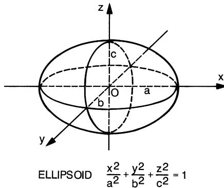
FIG. 7.5 The ellipsoid. (From Ayers, F., Jr., Theory and Problems of First Year College Mathematics , p. 387, ©1958, Schaum Publishing Co.: New York. This material is reproduced with permission of The McGraw-Hill Companies.)
