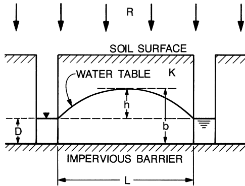
FIG. 7.7 Geometric representation of a homogeneous soil, underlain by an impervious barrier, that is drained by parallel, equally spaced ditches, where the ditches reach the impervious barrier, as considered by Hooghoudt. (From van der Ploeg et al., The Colding equation for soil drainage: Its origin, evolution, and use , ©1999, Soil Science Society of America: Madison, Wisconsin. Reprinted by permission of the Soil Science Society of America.)
