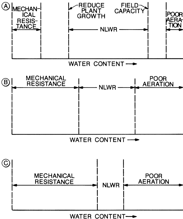
FIG. 8.3 Generalized relationships between soil water content and restricting factors for plant growth in soils with increasing bulk density and decreasing structure in going from case A to C. The non-limiting water range is abbreviated NLWR. (From Letey, J., Relationship between soil physical properties and crop production. Adv Soil Sci 1; 277-294, Fig. 4, 1985 ©Springer-Verlag, Heidelberg, Germany. This figure is used by permission of Springer-Verlag and John Letey.)
