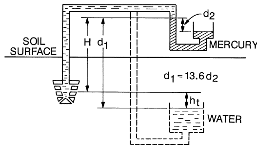
FIG. 4.2 Equivalent water and mercury tensiometers. (From Advanced Soil Physics by Kirkham, D., and Powers, W.L., p. 30, ©1972, John Wiley & Sons, Inc.: New York. This material is used by permission of John Wiley & Sons, Inc. and William L. Powers.)
