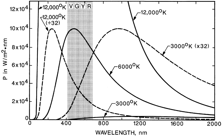
FIG. 23.8 The solid lines show plots of black-body radiation curves for temperatures of 3000, 6000, and 12,000°K. Broken lines show the 3000°K curve with ordinates multiplied by 32 and the 12,000°K curve with ordinates divided by 32; this adjustment brings the maxima of these curves to the same value as the maximum of the 6000°K curve. (From Shortley, G., and Williams, D., Elements of Physics , 5th ed., p. 844, ©1971. Reprinted by permission of Pearson Education, Inc: Upper Saddle River, New Jersey.)
