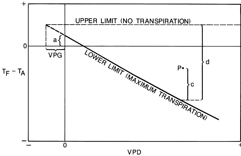
FIG. 25.9 The general form of the relationship between foliage-air temperature differential ( T_f - T_a ) and air vapor pressure deficit ( VPD ) for a stand of vegetation sufficiently supplied with water to transpire at the potential rate, i.e., the lower limit (maximum transpiration line), plus an illustration of how the upper limit (no transpiration line) is derived using the vapor pressure gradient ( VPG ). The values c and d are used to define the plant water stress index. See text for explanation. (From Idso, S.B., Reginato, R.J., and Farah, S.M., Soil- and atmosphere-induced plant water stress in cotton as inferred from foliage temperatures. Water Resources Research 18(4); 1143-1148, ©1982, American Geophysical Union. Reproduced by permission of American Geophysical Union.)
