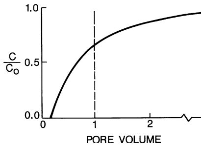
FIG. 12.8 Breakthrough curve characteristic of an unsaturated soil. (From Advanced Soil Physics by Kirkham, D., and Powers, W.L., p. 386, ©1972, John Wiley & Sons, Inc.: New York. This material is used by permission of John Wiley & Sons, Inc. and William L. Powers.)
