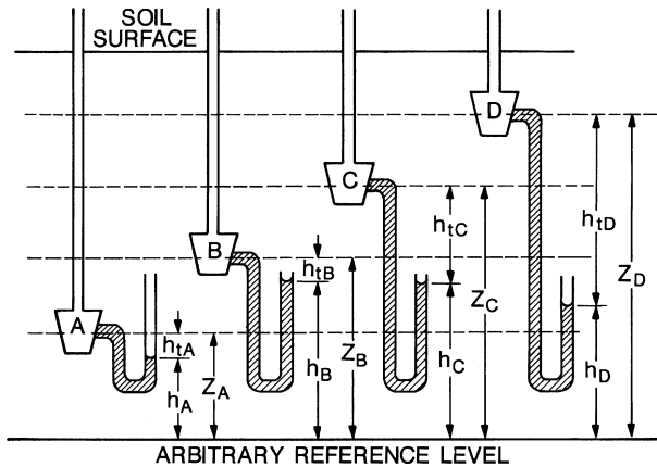
FIG. 5.3 Diagram to illustrate water movement between tensiometers. (From Advanced Soil Physics by Kirkham, D., and Powers, W.L., p. 240, 1984, Reprint edition, Robert E. Krieger Pub. Co.: Malabar, Florida; ©1972, John Wiley & Sons, Inc.: New York. This material is used by permission of John Wiley & Sons, Inc. and William L. Powers.)
