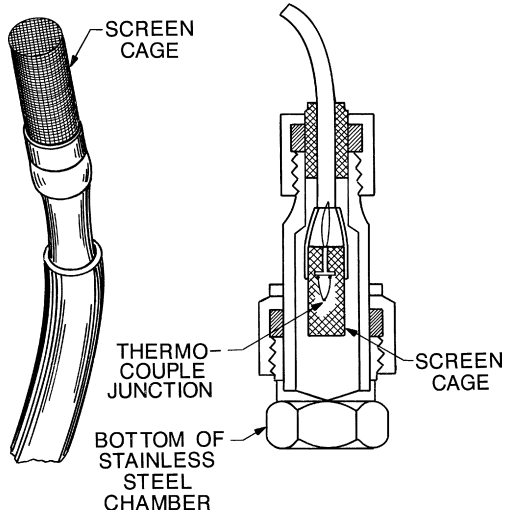
FIG. 16.8 Screen cage psychrometer. (From a figure in a brochure from J.R.D. Merrill Specialty Equipment, Logan, Utah.)
