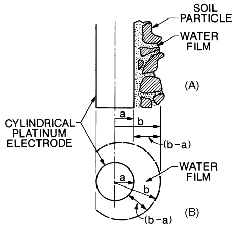
FIG. 10.4 The model that is assumed in order to explain microelectrode behavior. (A) Particles and solution separating the electrode from gas-filled pores. (B) Coaxial cylindrical model with water film of mean thickness (b - a) . (From Phene, C.J., ©1986, American Society of Agronomy and Soil Science Society of America: Madison, Wisconsin. Reprinted by permission of the American Society of Agronomy.)
