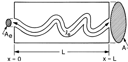
FIG. 10.5 Diffusion section model relating the actual path length ( l_e ) and area ( A_e ) to the block length ( L ) and cross section ( A ). (From Gaseous diffusion equation for porous materials by Troeh, F.R., Jabro, J.D., and Kirkham, D., Geoderma 27; 239–253, ©1982, Elsevier Scientific Publishing Co.: Amsterdam. Reprinted by permission of Elsevier, Amsterdam.)
