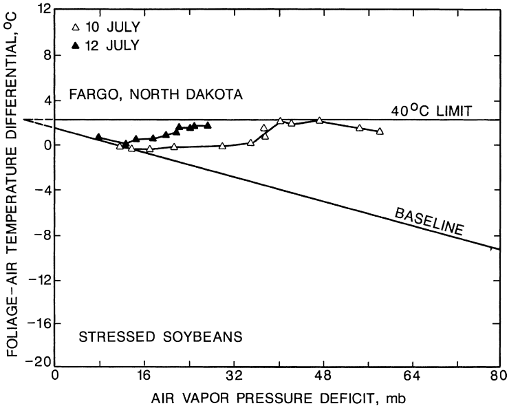
FIG. 25.11 Foliage-air temperature differential vs. air vapor pressure deficit for stressed soybeans growing at Fargo, North Dakota. (From Idso, S.B., Jackson, R.D., Pinter, Jr., P.J., Reginato, R.J., and Hatfield, J.L., Normalizing the stress-degree-day parameter for environmental variability. Agricultural Meteorology 24; 45-55, ©1981, Elsevier Scientific Publishing Company: Amsterdam. Reprinted by permission of Elsevier, Amsterdam.)
