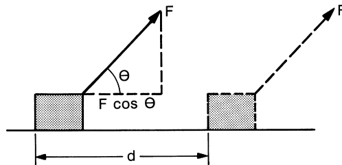
FIG. 2.1 Illustration for definition of work. (Adapted from Schaum D., Theory and Problems of College Physics , p. 49, ©1961, Schaum Publishing Co., New York. This material is reproduced with permission of The McGraw-Hill Companies.)
