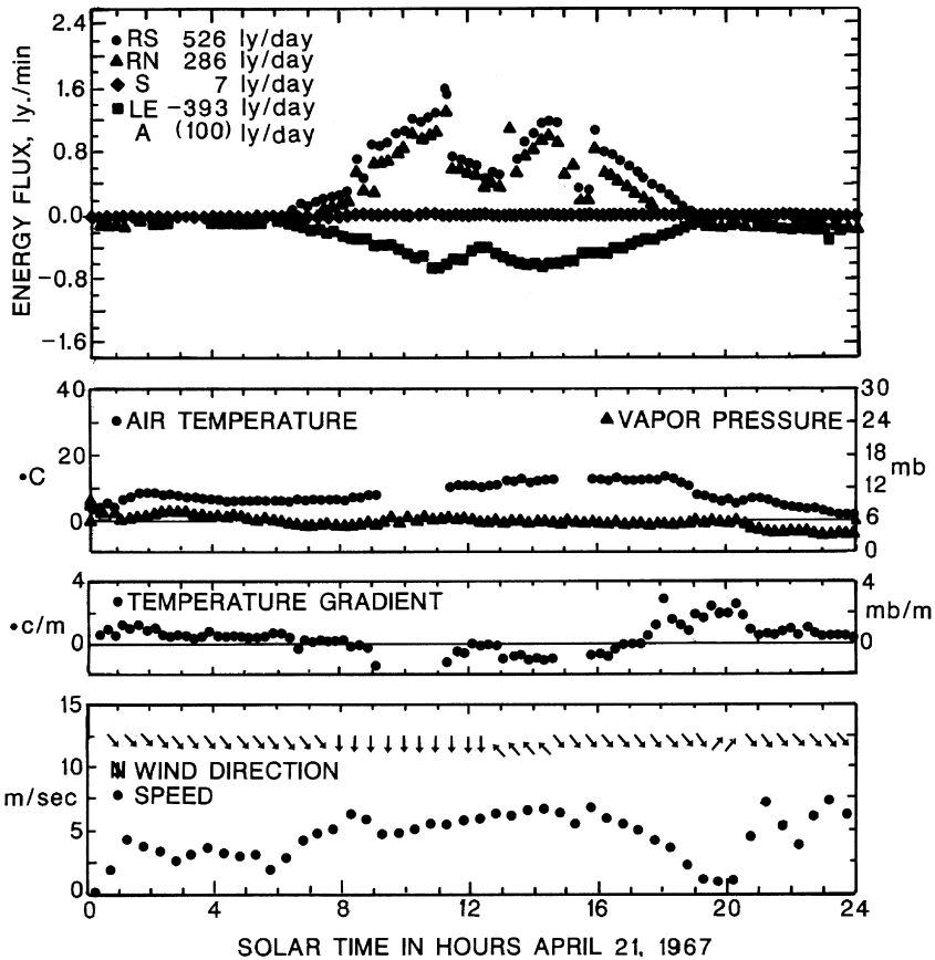
FIG. 26.4 Energy balance with lysimetrically measured evapotranspiration from alfalfa at Mead, Nebraska, April 21, 1967. Air temperature and vapor pressure measured at 100 cm; gradients between 45 and 100 cm; wind speed at 200 cm. RS = solar radiation; RN = net radiation; S = soil heat flux; LE = evaporation; A = sensible heat flux. (From Rosenberg, N.J., Microclimate: The Biological Environment , p. 174, ©1974, John Wiley & Sons, Inc: New York. This material is used by permission of John Wiley & Sons, Inc.)
