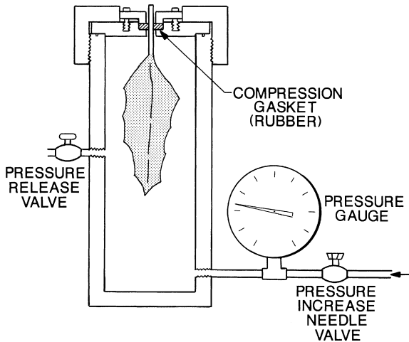
FIG. 17.2 Diagrammatic cross section through a pressure chamber for measurement of leaf water potential by pressure equilibration. (From Kramer, P.J., Water Relations of Plants , p. 385, ©1983, Academic Press: New York. Reprinted by permission of Academic Press.)
