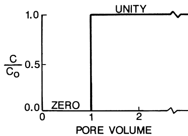
FIG. 12.5 Breakthrough curve for piston flow. (From Advanced Soil Physics by Kirkham, D., and Powers, W.L., p. 385, ©1972, John Wiley & Sons, Inc.: New York. This material is used by permission of John Wiley & Sons, Inc. and William L. Powers.)
