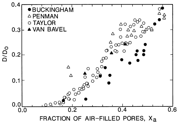
FIG. 10.2 Scatter diagram of the relation between the ratio D/D_0 and the fraction of air-filled pores x_a calculated from data of Buckingham (1904) (closed circles), Penman (1940) (open triangles), Taylor (1949) (open circles), and van Bavel (1952) (closed triangles). D_0 is the coefficient of diffusion of \text{CO}_2 in still air. D is the coefficient of diffusion of \text{CO}_2 in the soil. If x_a decreases to 0.1 to 0.2, D appears to become zero. (From Wesseling, J., and van Wijk, W.R., ©1957, American Society of Agronomy: Madison, Wisconsin. Reprinted by permission of the American Society of Agronomy.)
